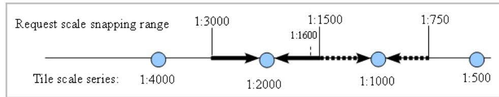
Figure 2-9 snap_to_tile_scale Attribute
