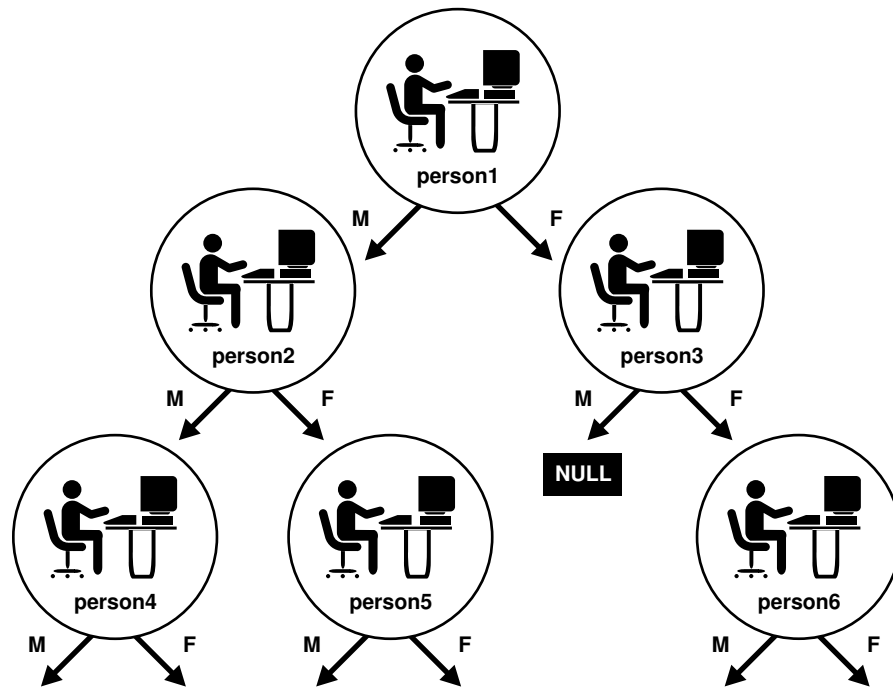
Figure 22-2 Object Graph of person_t Instances
