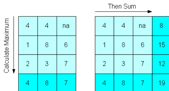
Figure 9-6 Max Method Followed by Sum Method
