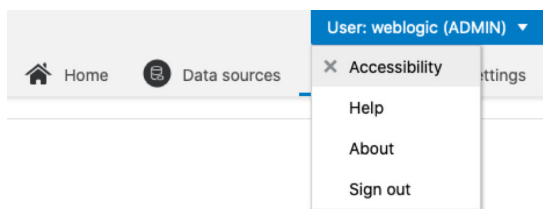
Figure 11-46 Disabled Accessibility
