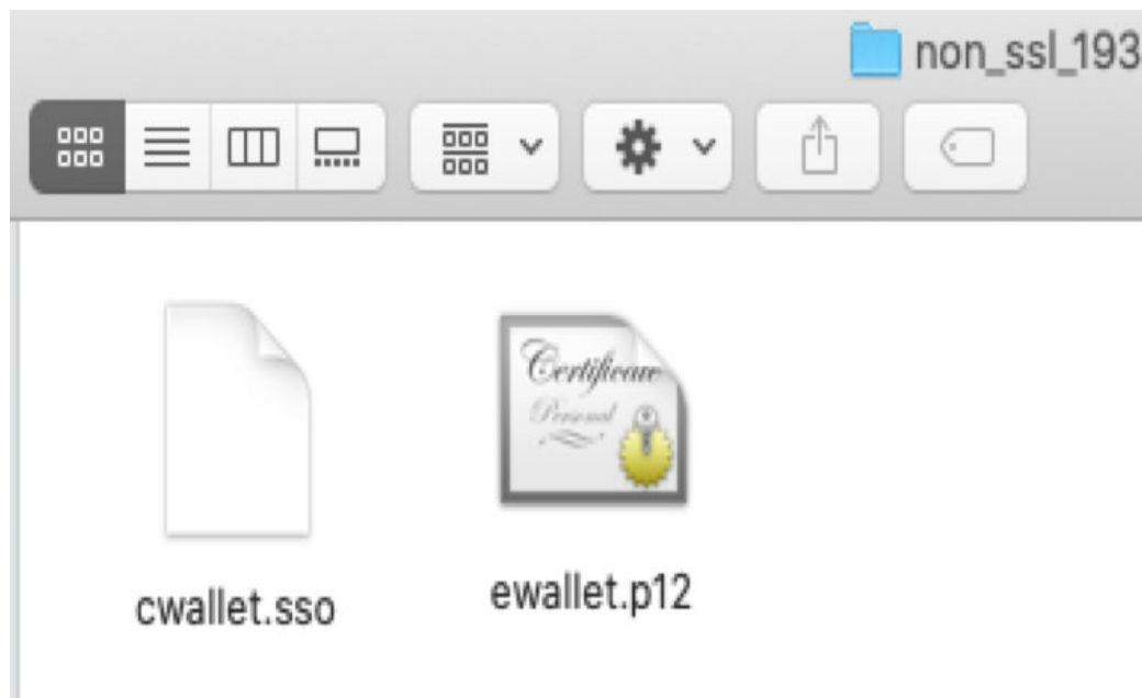
Figure 11-19 Simple Wallet
