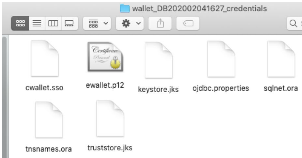
Figure 11-20 Cloud Wallet
