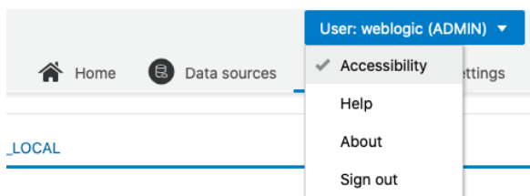
Figure 11-47 Enabled Accessibility
