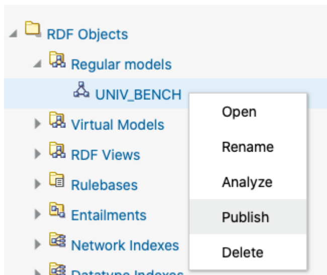
Figure 11-36 Publish Menu
