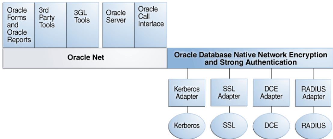
Figure 19-4 Oracle Net Services with Authentication Adapters
