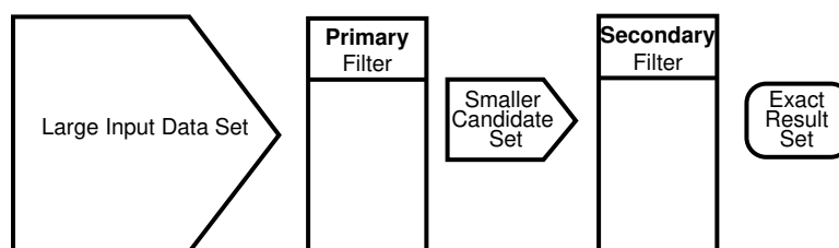
Figure 1-2 Query Model
